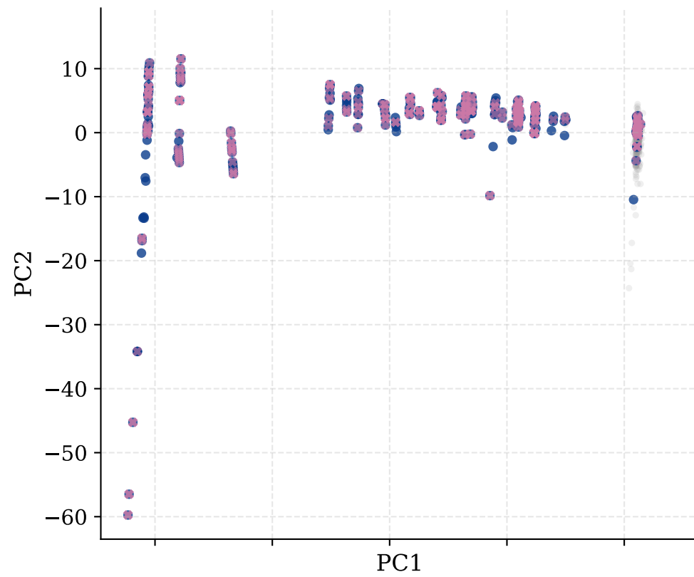
CTGAN
