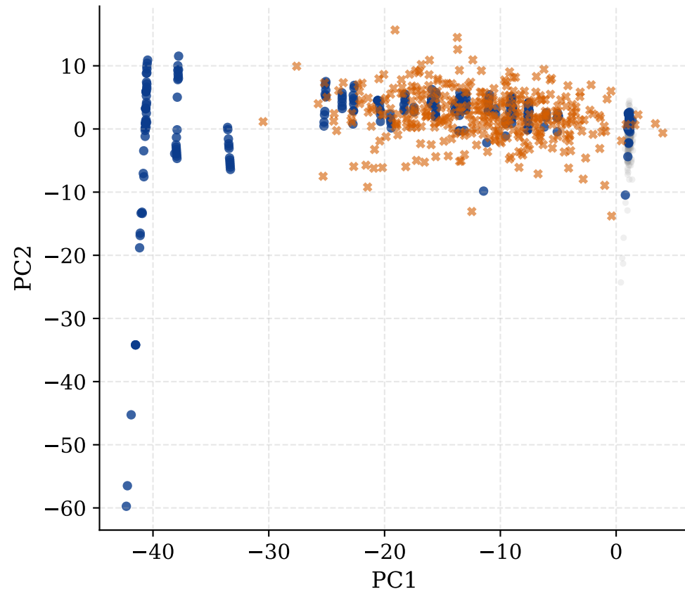
CTGAN
